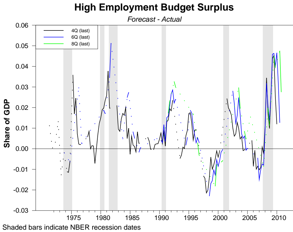
FIGURE 8. HEB - FORECAST ERRORS (WITH NBER BUSINESS CYCLE DATES)
