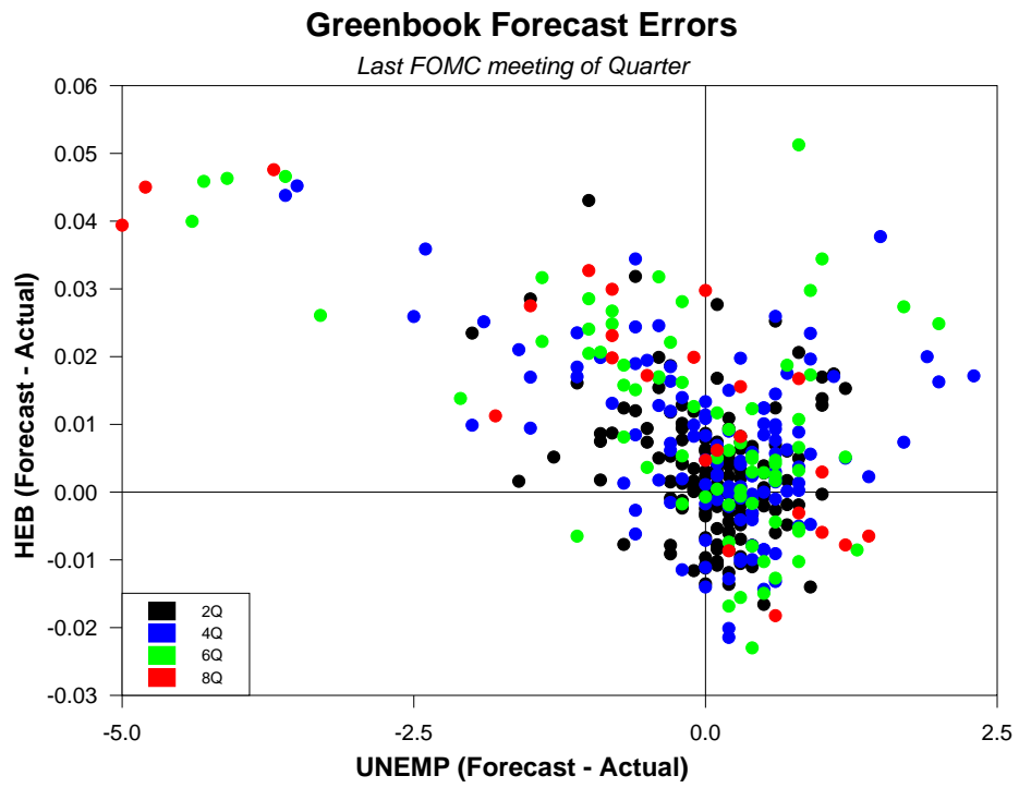
FIGURE 9. HEB - FORECAST ERRORS AT BUSINESS CYCLE TROUGHS
